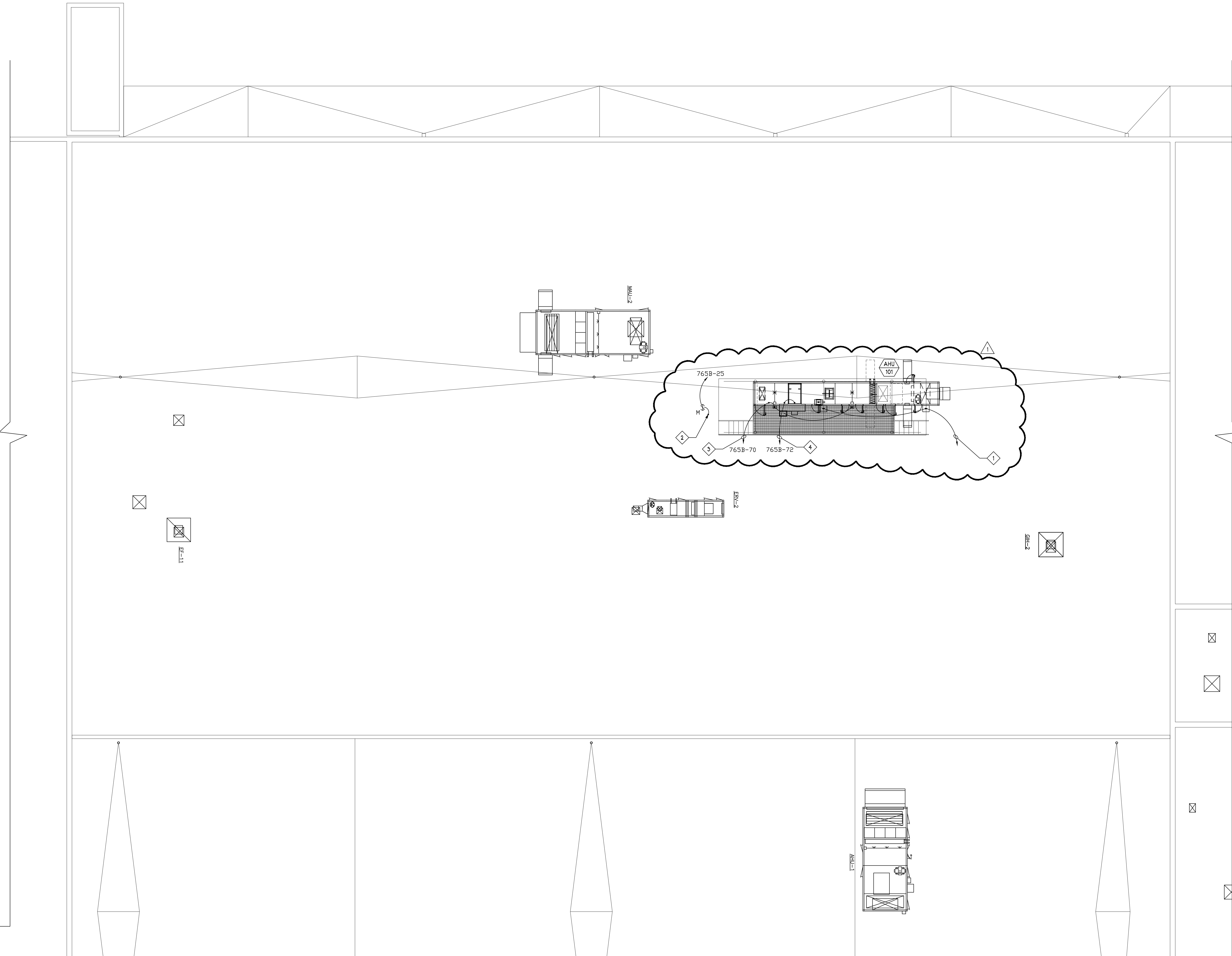
ROOF POWER PLAN 1/8" = 1'-0"
