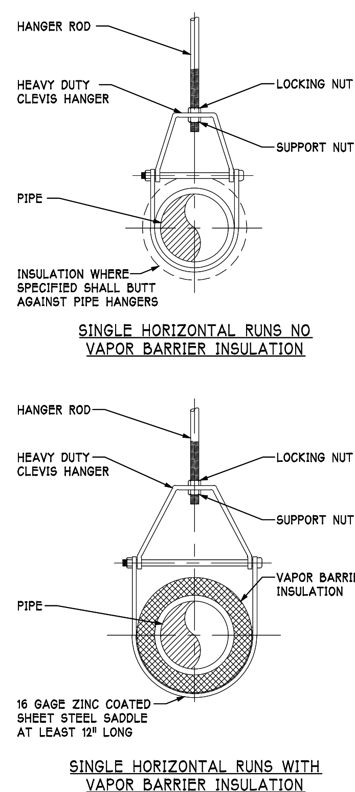
CLEVIS HANGER DETAIL
