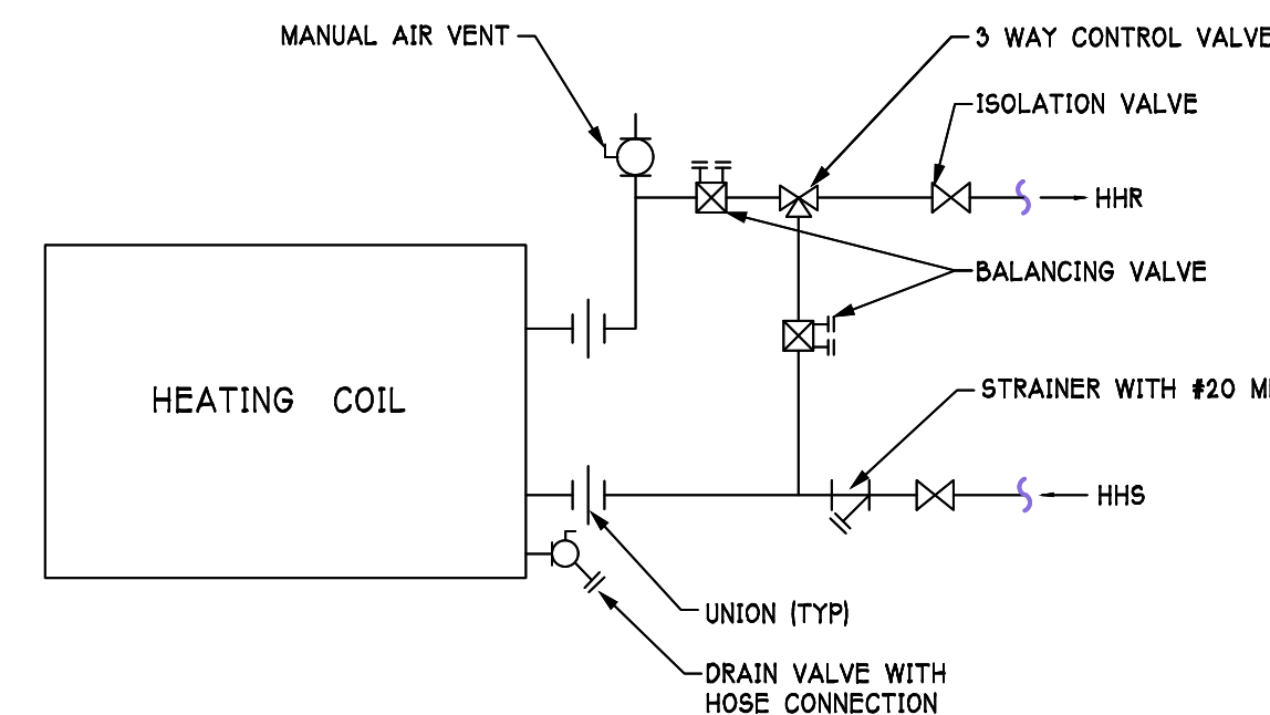
COOLING COIL PIPING DETAIL
