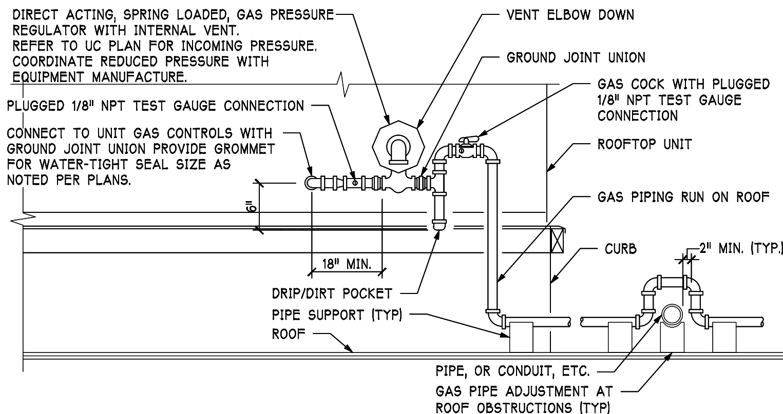
TYPICAL ROOFTOP UNIT GAS PIPING CONNECTION DETAIL
