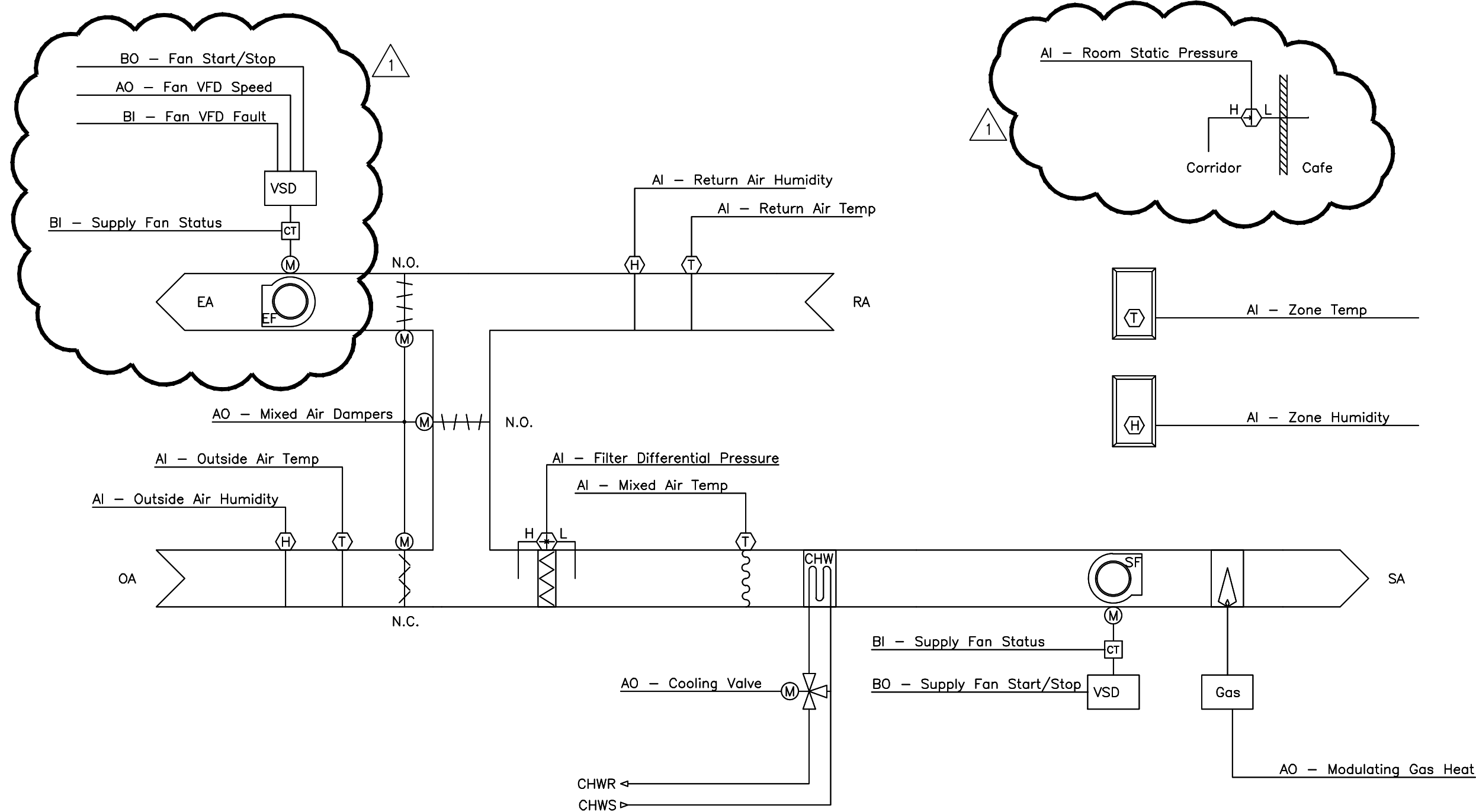
AHU-101 CONTROL SCHEMATIC
