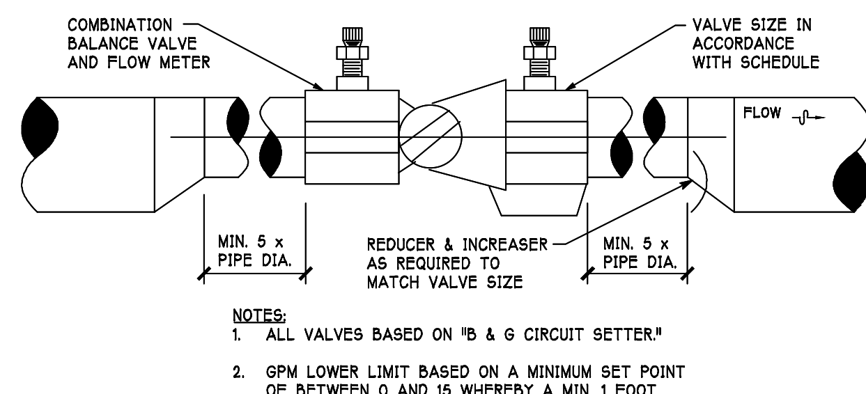
CIRCUIT SETTER DETAIL
